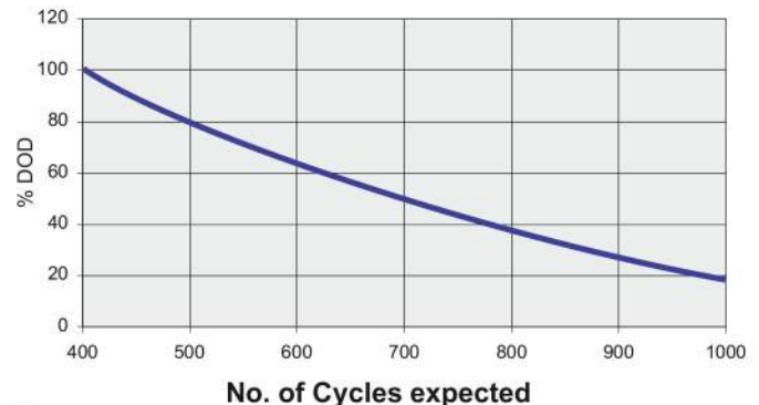
Cycle life Vs Depth of Discharge
